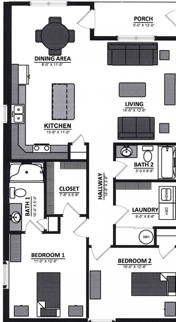
Luxury Level (First Floor)
