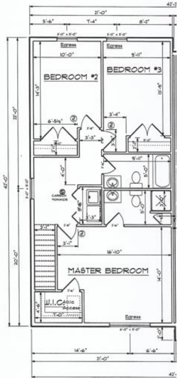
Second Floor
