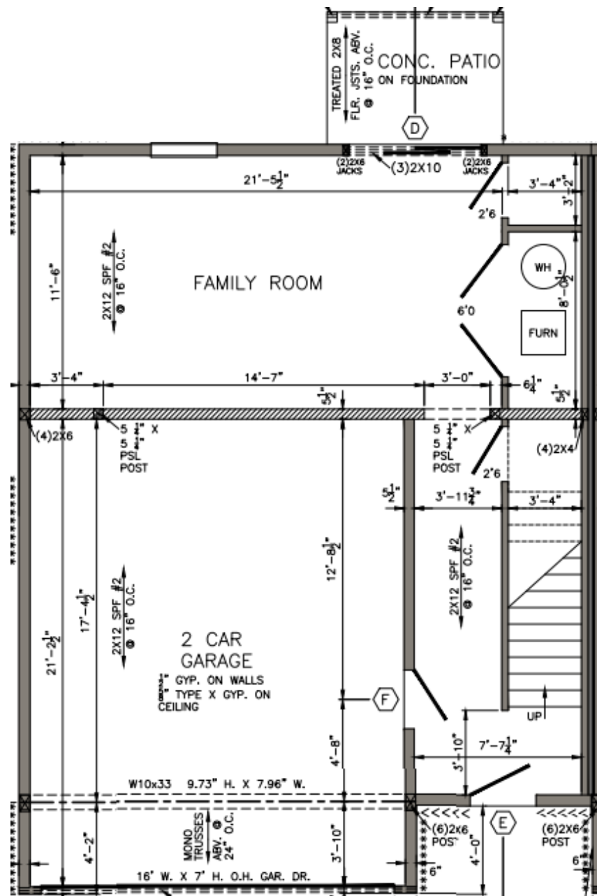
Basement/Entry Level
